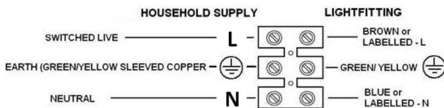
WIRING DETAILS
