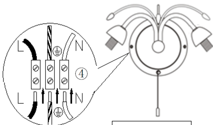
WIRING DETAILS
